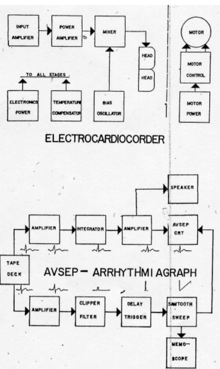
Fig. 5. Block diagram of the recorder-analyzer system.
